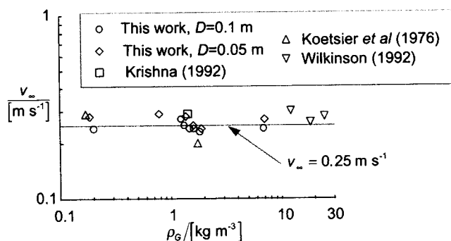
Figure 6. Single-bubble rise velocity as a function of gas density for the experimental investigations in Table 1.
